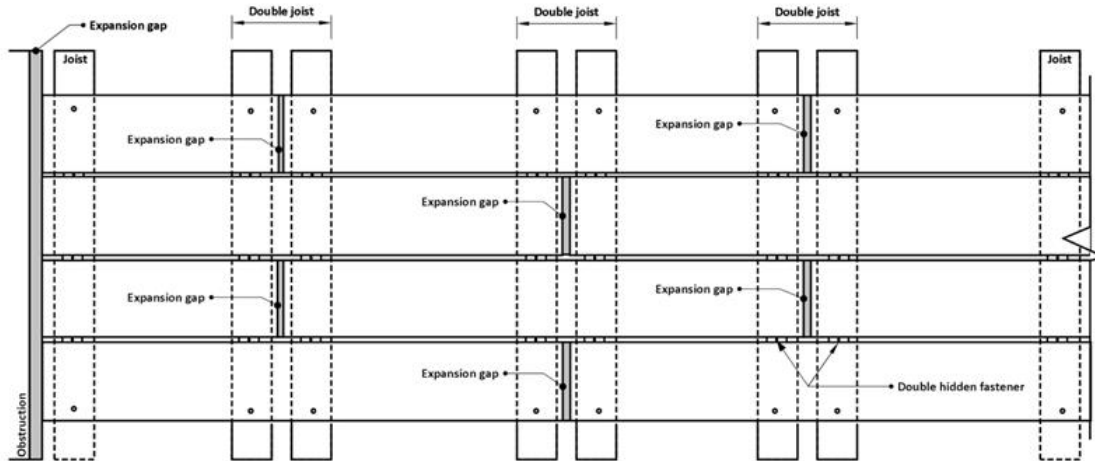
Staggered laying pattern
